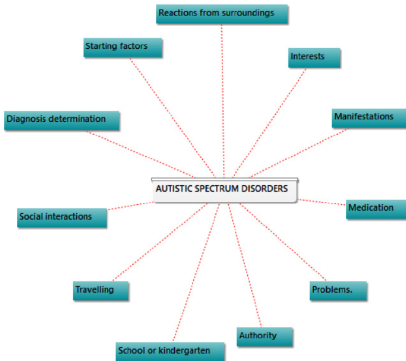
Scheme 4: ASD
